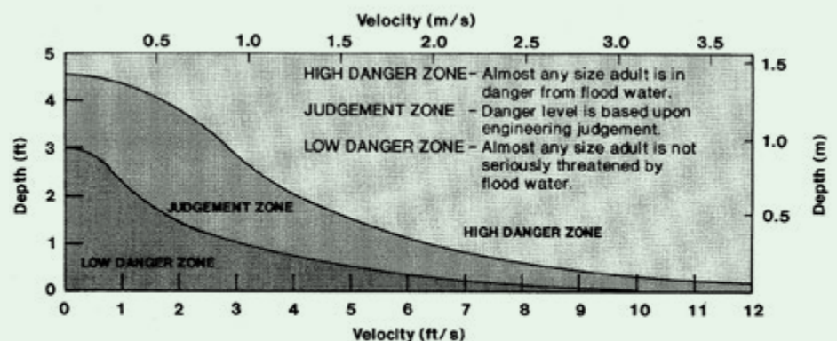
Figure 5. – Depth-velocity flood danger level relationship for adults.
